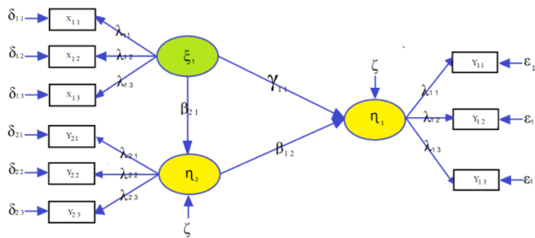
Gambar.1 Model Statistik
